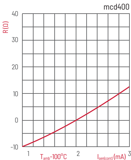
Fig 4. Deviation of sensor resistance as a function of operating current in still liquid
